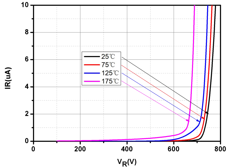
Fig.2-Typical Reverse Characteristics
