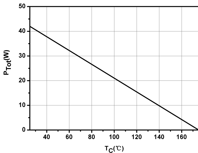
Fig.7-Power Derating
